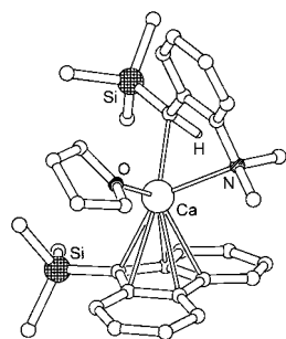
Figure 1. The crystal structure of 3 (only one of the two crystallographical independent but isostructural molecules is depicted). Hydrogen atoms (except for the benzylic hydrogen) have been omitted for clarity. Selected bond lengths [Å] for both independent molecules: Ca–C \alpha : 2.501(2) and 2.510(2); Ca–N: 2.462(2) and 2.470(2); Ca–O: 2.305(2) and 2.310(2); Ca–fluorenyl contacts: 2.690(2), 2.733(2), 2.736(2), 2.785(2), 2.789(2) and 2.683(2), 2.732(3), 2.724(2), 2.771(2), 2.778(2).
